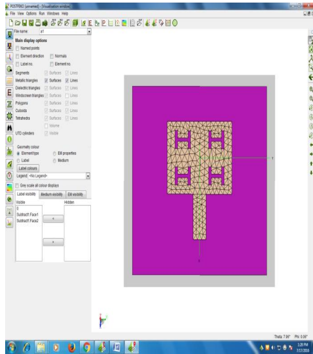
Fig.3 In the fig.3 show the meshing of the patch. The dimension of the antenna is 40*50, and dimensions of slot are 10*10.
