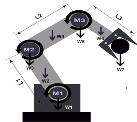
Figure 3 : FBD of Robotic arm
