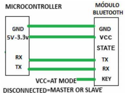
Figure 5 : Application Circuit
