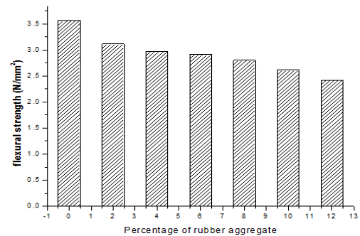
Fig 3.4 Variation of flexural strength with addition of rubber aggregate
