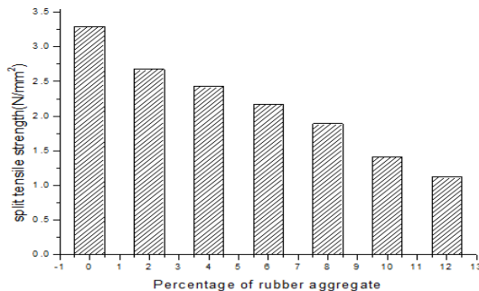
Fig 3.3 Variation of split tensile strength with addition of rubber aggregate
