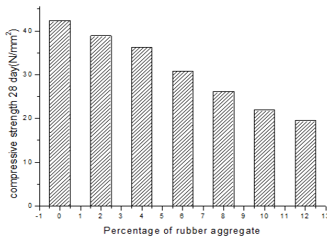
Fig 3.2 Variation of compressive strength (28 day) with addition of rubber aggregate
